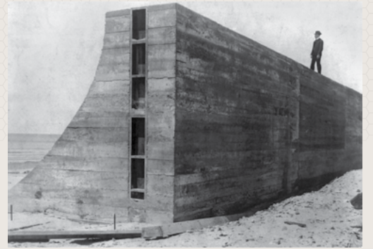
Construction of the Galveston Seawall
